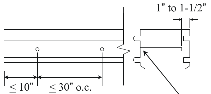
Figure 2. Drilling Detail
