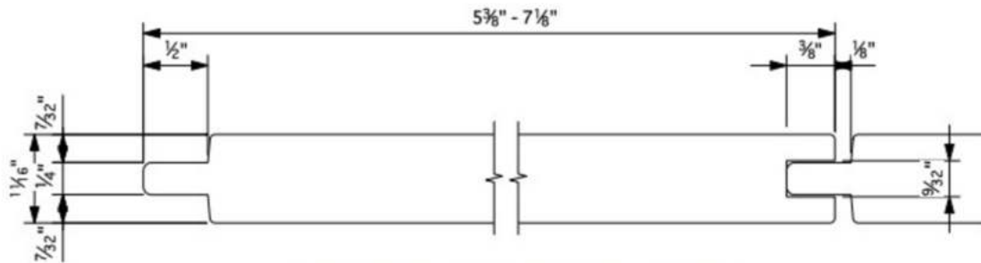
Elite Finline (1/8 th Gap) Paneling
